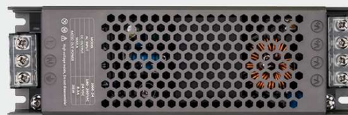
844529 200W 24V 8,3A 188 x 60 x 30 mm
