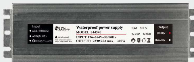
844540 300W 24V 12,5A 257 x 73 x 45 mm
